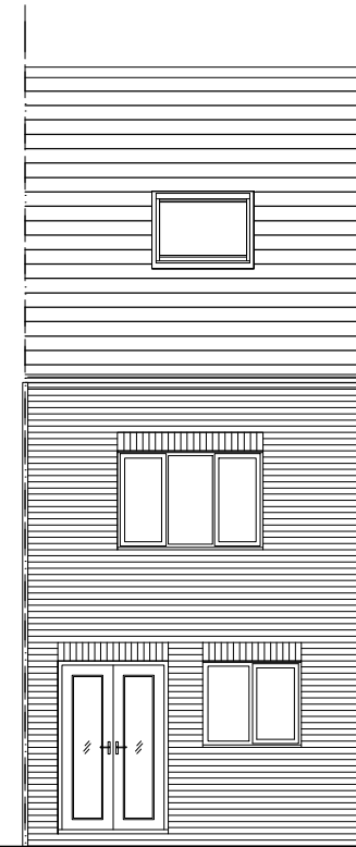
Rear Elevation
